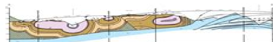
GEOLOGIC MAP OF THE HOCKBACK MOUNTAIN QUADRANGLE, LEWIS AND CLARK AND MENAGER COUNTRIES, MONTANA
