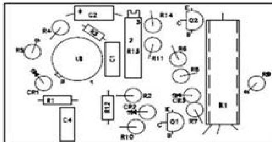
B. PRINTED CIRCUIT BOARD LAYOUT DIAGRAM
