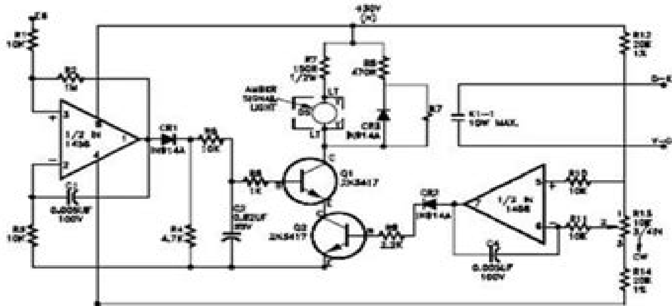
A. CIRCUIT SCHEMATIC DIAGRAM
