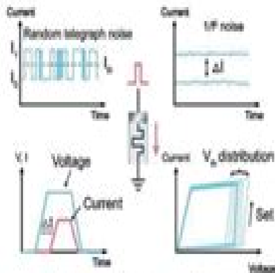
Stochastic computing
