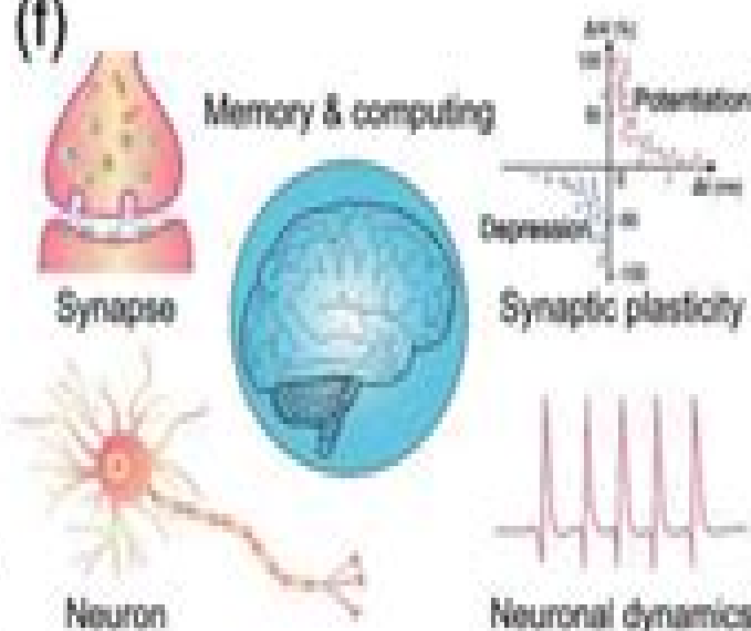
Brain-inspired computing
