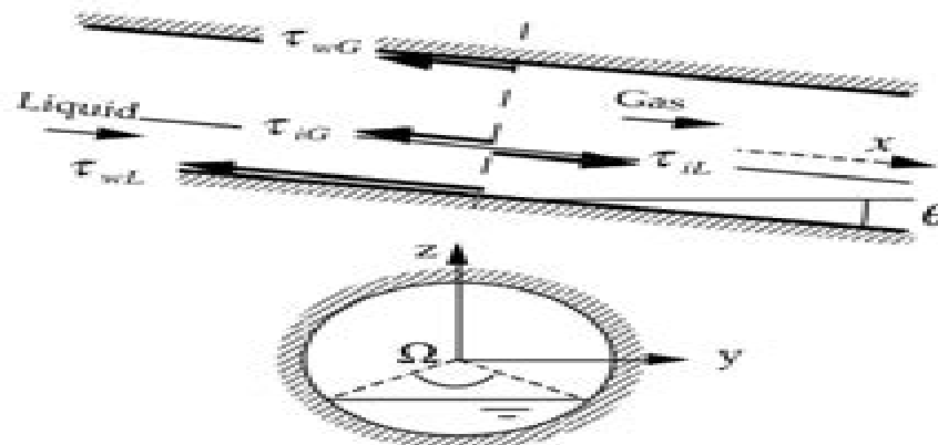
Figure 1. Gas-liquid stratified flow
