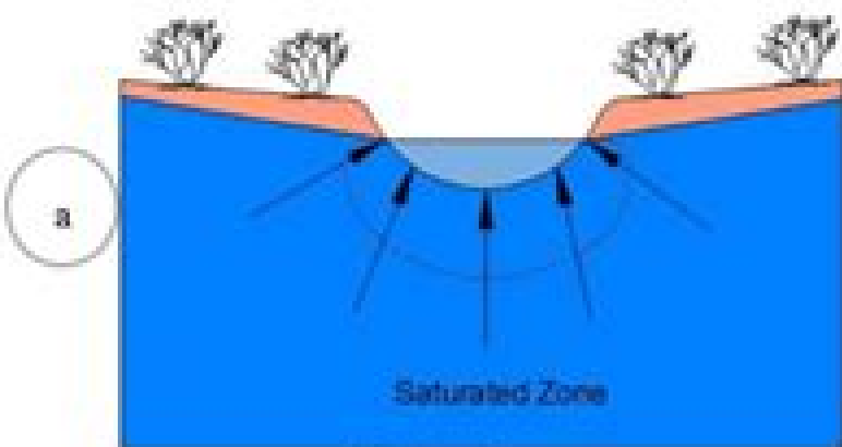
Gaining Stream
