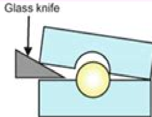
(2) Fracture with a glass knife
