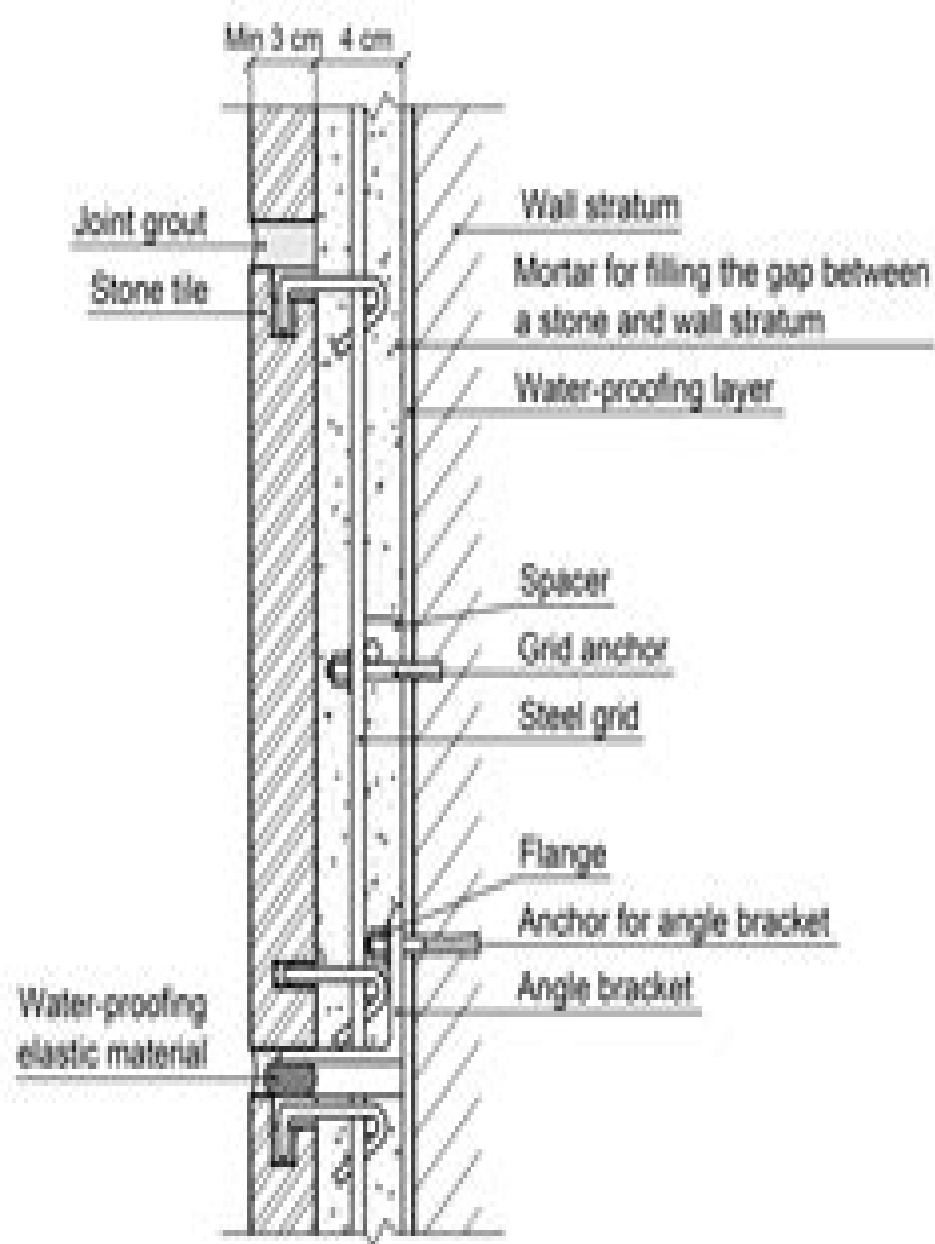
Wet-fixed stone cladding
