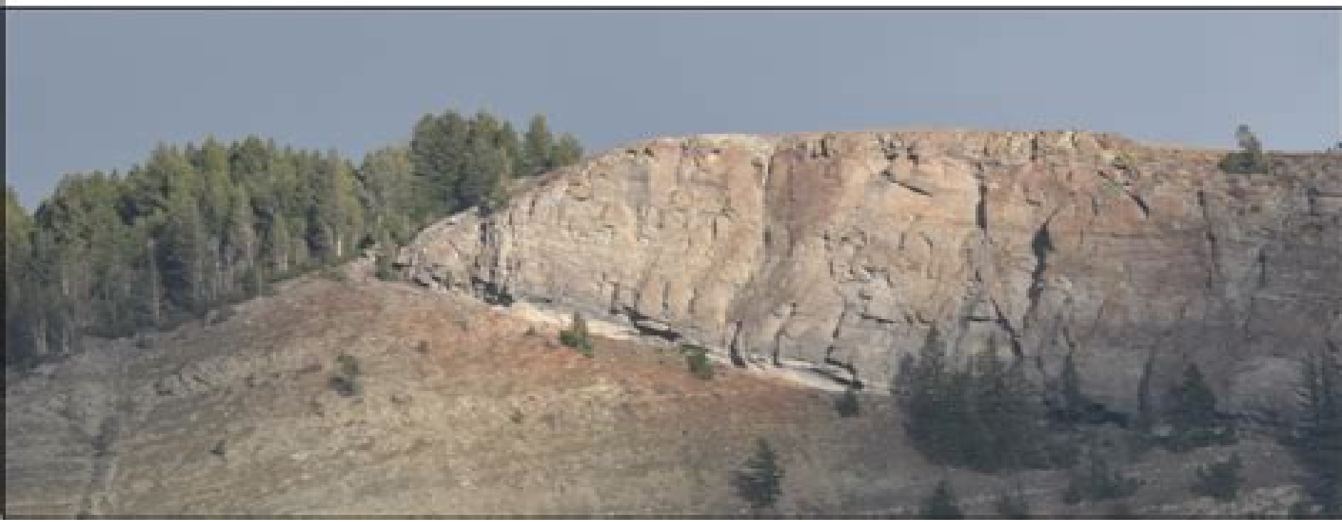
Plate VII. —Showing contact of rhyolite cap of Mount Evarts with the Cretaceous sandstones.
