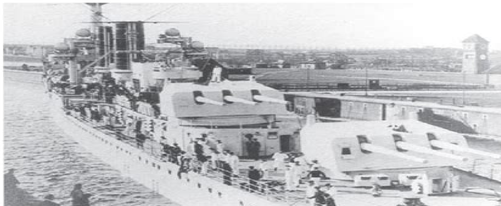
Karlruhe in a Wilhelmshaven lock after commissioning. Notice the dark-painted funnels. The photograph gives a good view of the unorthodox alignment of 'B' and 'C' turrets off the centreline. In accordance with German naval tradition, 'C' turret bore the name SMS Goeben .
