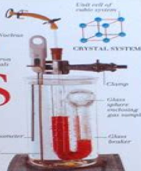
CHARLES LAW
