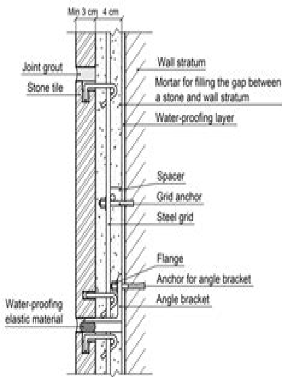
Wet-fixed stone cladding
