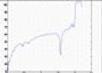
Restored spectrum
