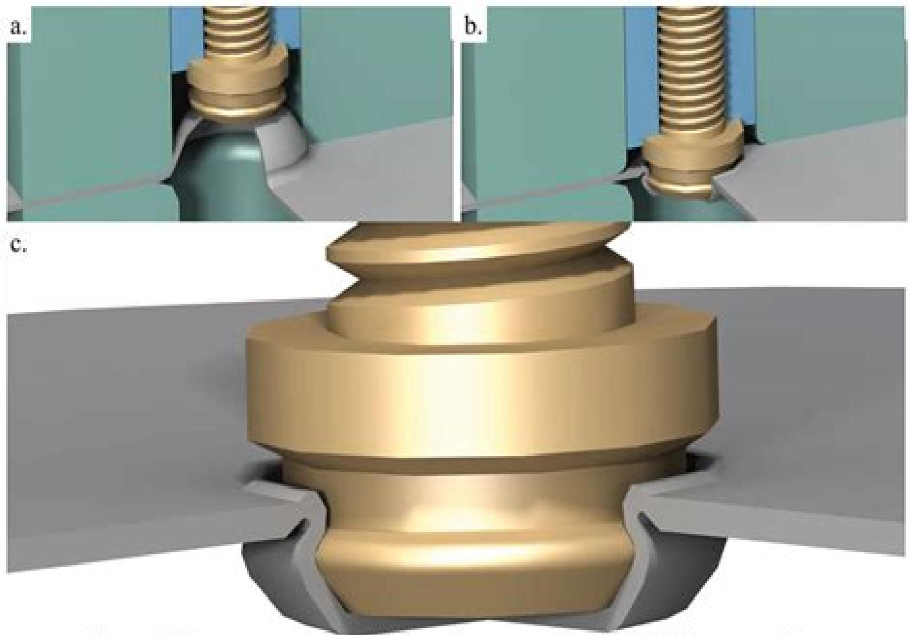
Figure 1: 3Fs process step – (a) forming operation, (b) folding operation, (c) cross-section view of fastener and sheet metal at the end of the process
