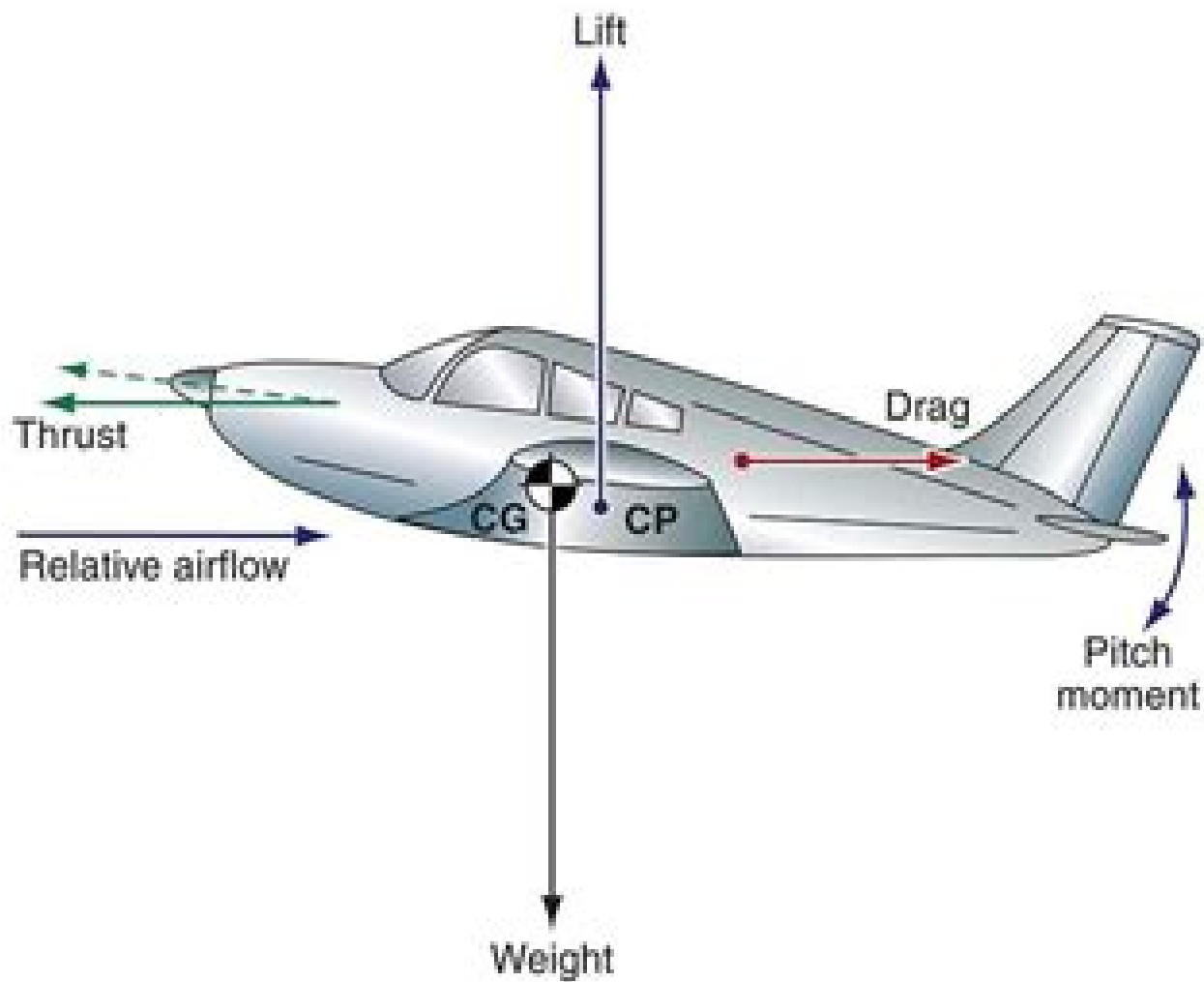
Figure 3-1. Balance of forces and moments.
